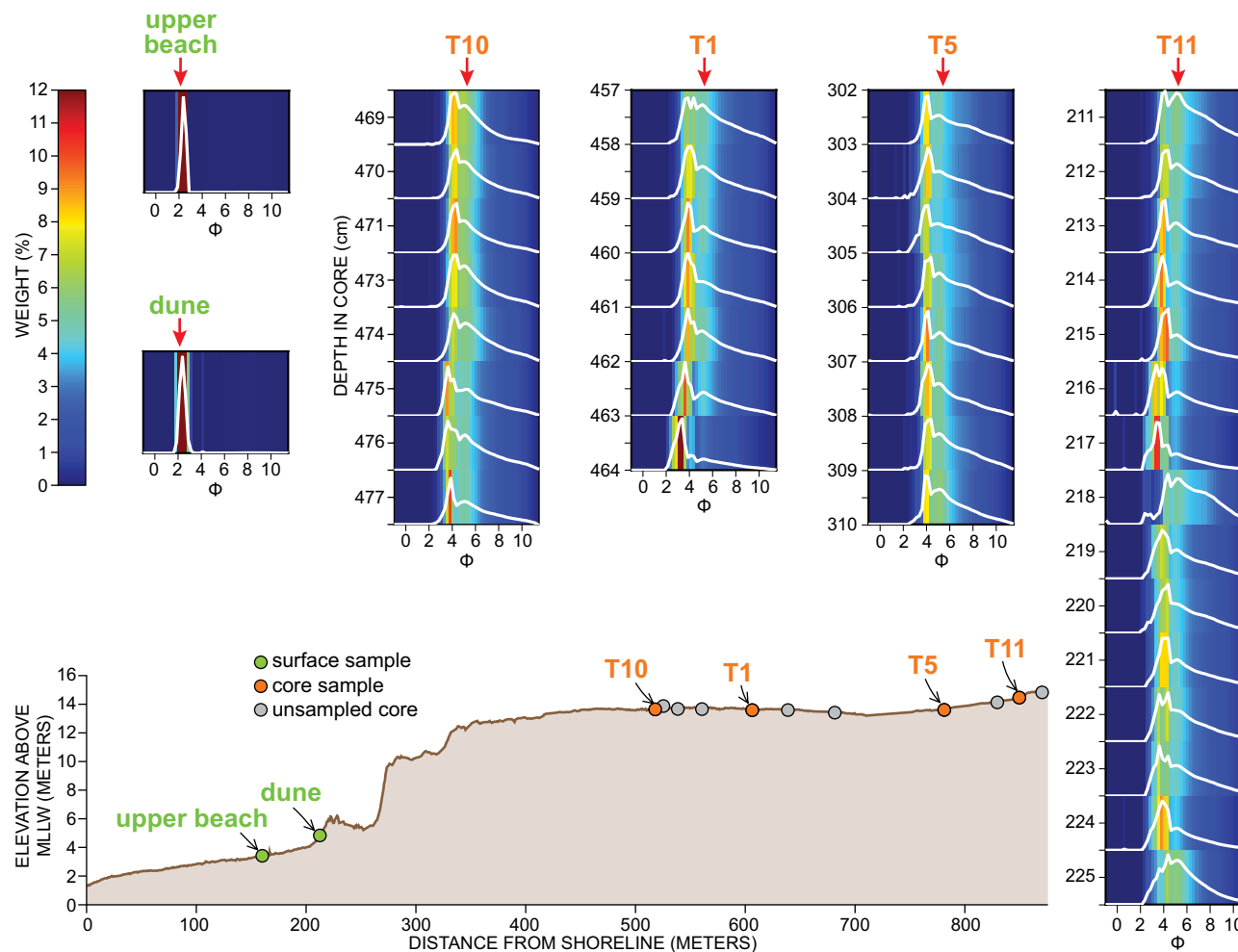
Figure 7. Changes in grain-size distribution in bed C' among four cores (orange labels) on the Tsunami Ramp core transect. Vertical red arrows mark mean grain-size distribution of the bed in the four cores. Grain-size distributions for modern beach and dune samples, located along the elevational transect, are also shown. MLLW—mean lower low water.
