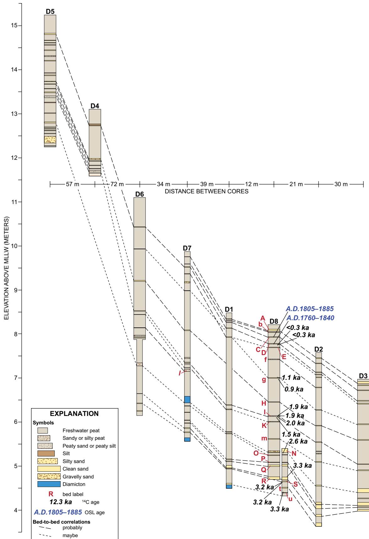
Figure 5. Correlation of axial cores at the Drained Lake site. Gouge cores (2.5 cm diameter; narrow columns) and Russian cores (5 cm diameter; wide columns) were described and photographed in the field. Core D8 was described and sampled in detail in the laboratory. Bed labels as in Table 2. Accelerator mass spectrometer 14 C ages are the mode of the calibrated probability age distribution rounded to the nearest century (Table 3). Data for optically stimulated luminescence (OSL) ages are in Table 4. MLLW—mean lower low water.
