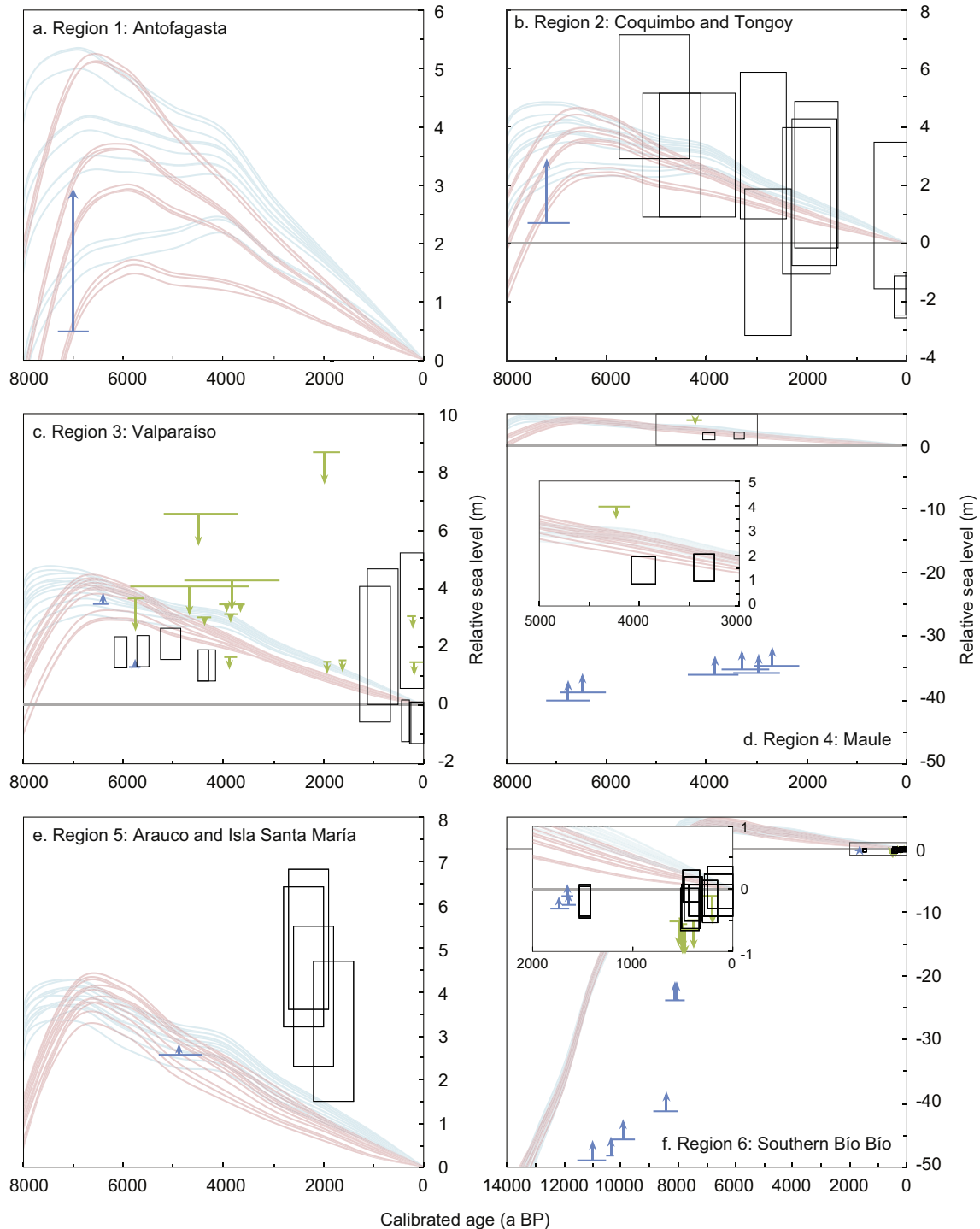
Fig. 7. Regional plots comparing the age – elevation distribution of the sea-level data points with glacial isostatic adjustment model predictions (following Peltier, 2004; Peltier et al., 2015). Sea-level index points are black rectangles, terrestrial and marine limiting points are green T-shaped symbols and blue L-shaped symbols respectively. ICE_5G predictions are light blue curves, ICE_6G predictions are pink curves; for both ice models we vary the lithospheric thickness between 71 and 120 km and the upper mantle viscosity between 5 \times 10^{19} Pa s and 2 \times 10^{20} Pa s (see section 3.7). Note different x-axis scaling for panel f and variable y-axis scaling between all panels. (For interpretation of the references to colour in this figure legend, the reader is referred to the Web version of this article.)
